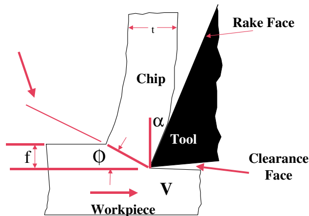
Figure 1. Idealized Chip Formation Process (Turning)
